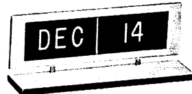
CR-260-S 6x1 \frac{1}{2} x2 \frac{3}{16} CR-260-D 6x2x2 \frac{3}{16}
